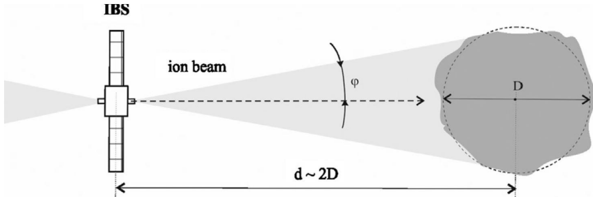
Fig. 8: Schematic diagram of the principle of the “ion-beam shepherd” deflection concept. A collimated beam of quasi-neutral plasma is directed at the asteroid surface. The spacecraft, placed at a distance of a few asteroid diameters, would need a second propulsion system to compensate for the ion engine reaction and keep a constant distance between the asteroid and the shepherd spacecraft. From Bombardelli et al., (2013).
