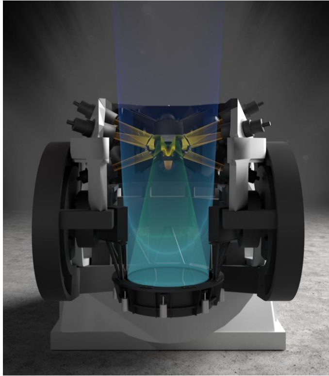
Fig. 5: Fly-eye concept. Credit: ESA/A. Baker
