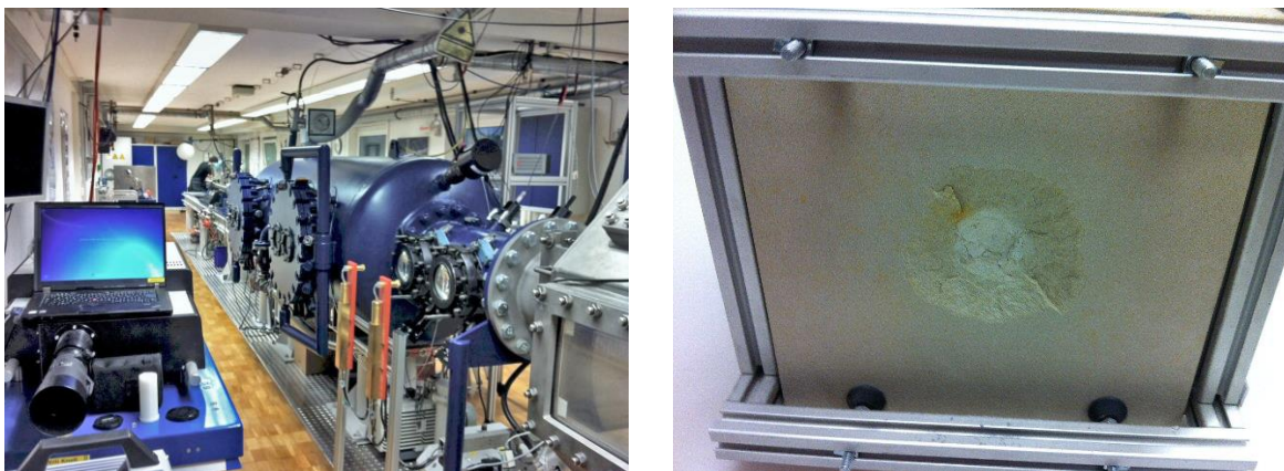
Fig. 7: Hypervelocity gas gun and target block of asteroid analog material, Fraunhofer Ernst Mach Institute, Freiburg, Germany. Credit: Alan Harris, NEOShield
